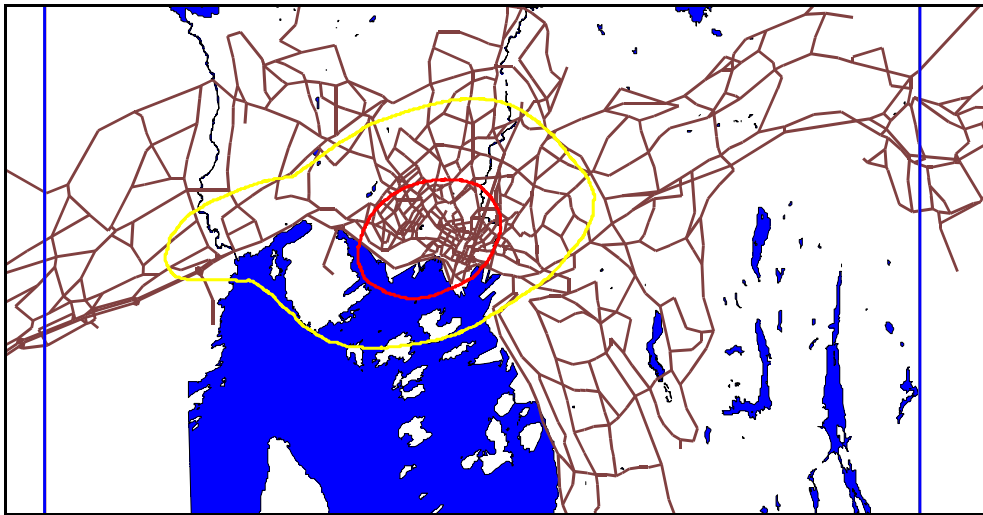
Figure 4: SO 2 concentrations for Oslo in 1995. Iso-lines for 3 and 5 µg/m 3 .
