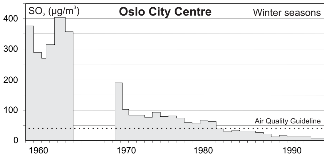
Figure 2: Winter concentration of SO 2 in Oslo city from 1958 to 1995. The Norwegian recommended Air Quality Guideline is given (Larssen, 1998).
