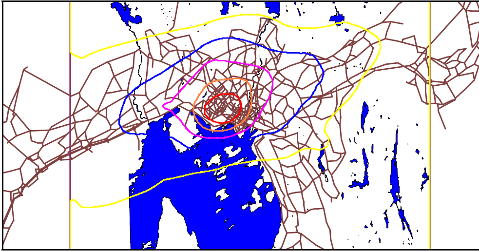
Figure 3: SO 2 concentrations for Oslo in 1979. Iso-lines for 5, 25, 35, 45, 55 µg/m 3 .
