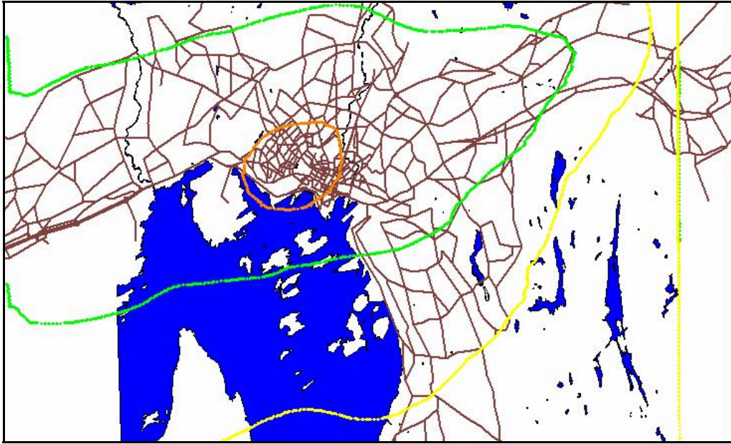
Figure 6: Lifetime for galvanised steel in 1979. The lifetime is defined as the time where the zinc coating was corroded away. The iso-lines are given for 30, 40 and 50 years. 30 years is in the centre of Oslo.
